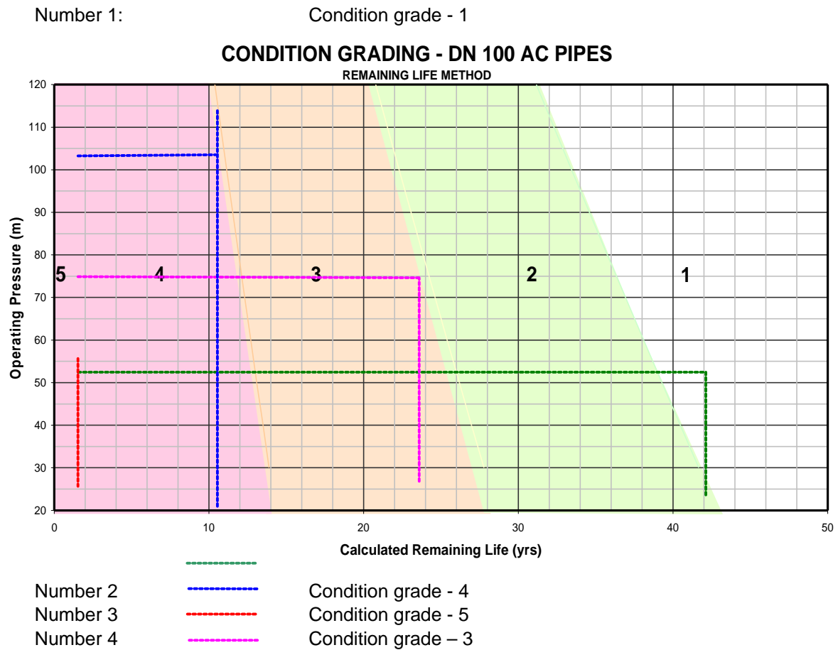
FIGURE 2-1 EXAMPLE OF PREDICTED REMAINING LIFE METHOD OF GRADING
