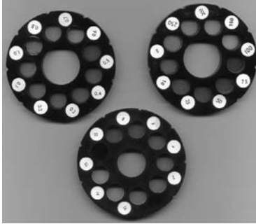
Lovibond comparator discs
