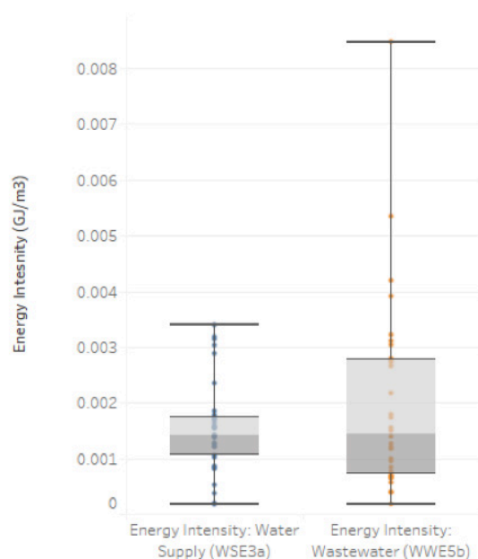
Figure 71: Energy intensity for water and wastewater systems
