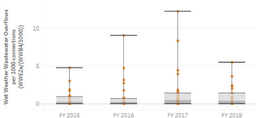
Figure 13: Trend showing maximum, minimum and median number of wet weather overflows per connections serviced
