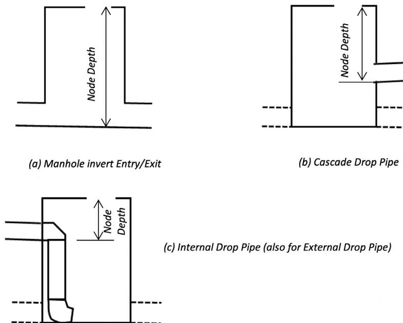
Figure B2.1_5, examples of typical situations and the measurements for the depth of node (depth of pipe)
