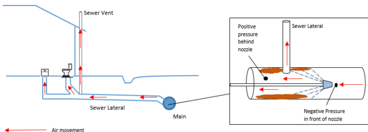
Figure B1.1.3 – Diagram showing how pressure causes blowbacks
